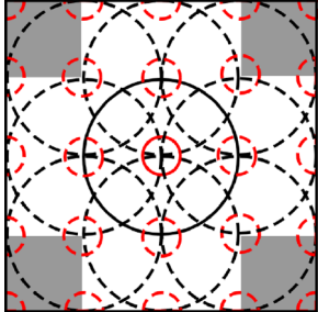
(b) Fourier support
