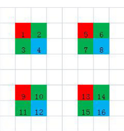
(a) subsampling
