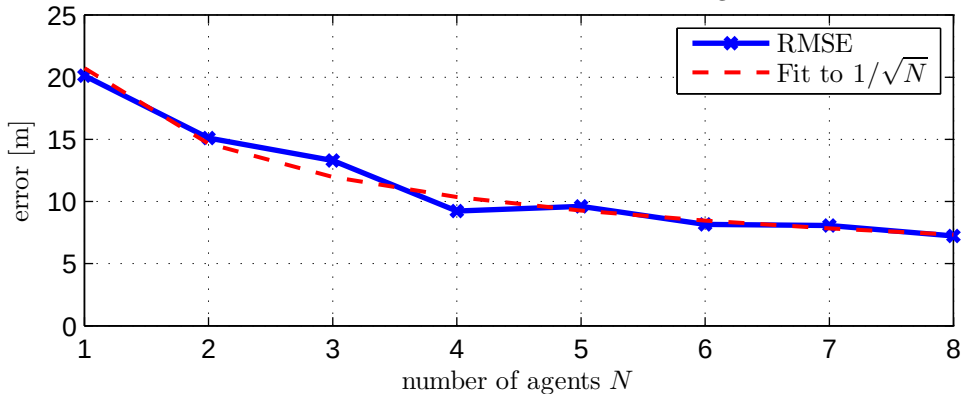
RMSE as a function of the number of agents
