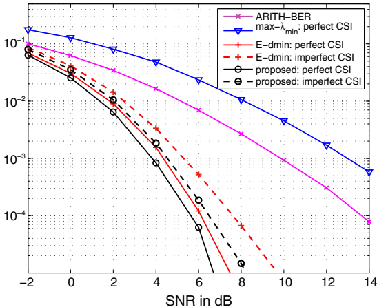
MIMO system (5,4) using 4-QAM modulation, imperfect CSI
