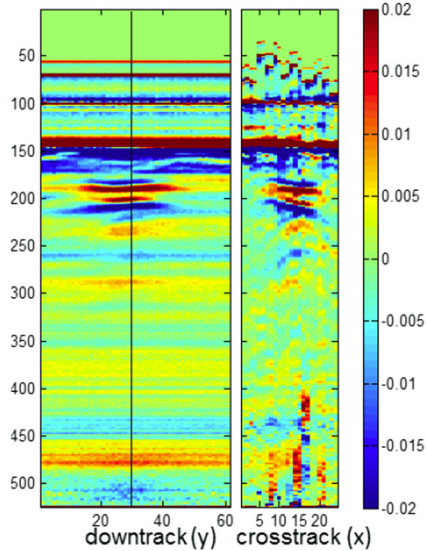
(c) Non-metalClutter
