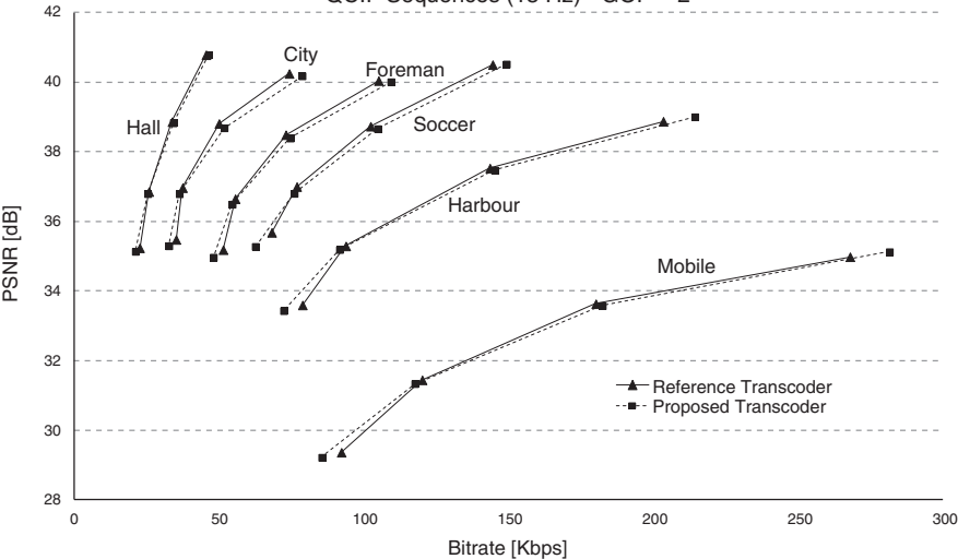
QCIF Sequences (15 Hz) - GOP = 4
