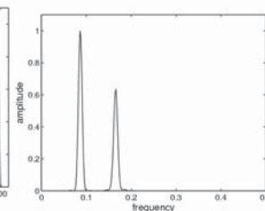
(i) frequency resolution, a=0.25
