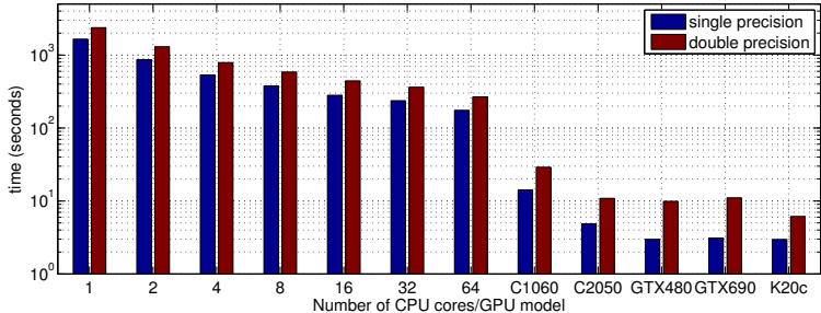
3D Shearlet compute times
