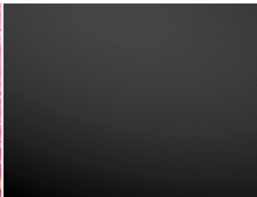
illumination model
