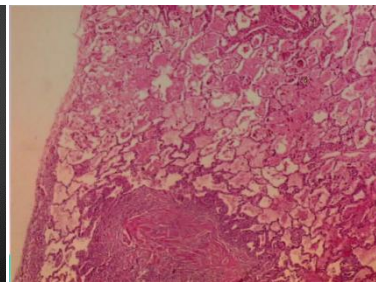
corrected image
