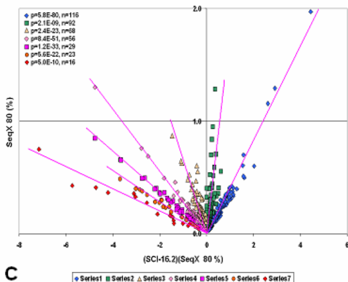
Amino Acid Co-locations vs. Size Compatibility Index
