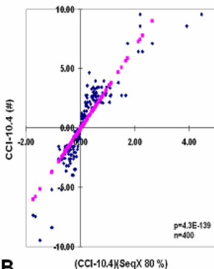
Amino Acid Co-locations vs. Size Compatibility Index
