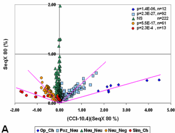
Amino Acid Co-locations vs. Size Compatibility Index
