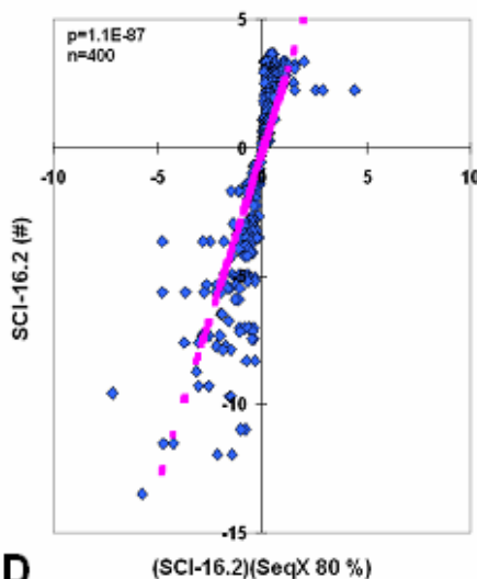
Amino Acid Co-locations vs. Size Compatibility Index
