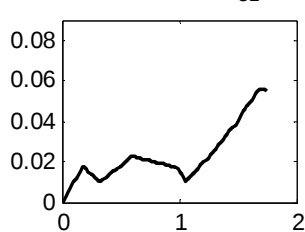
Glucose(N) r_{38}
