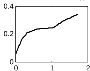
Glucose(A) r_1
