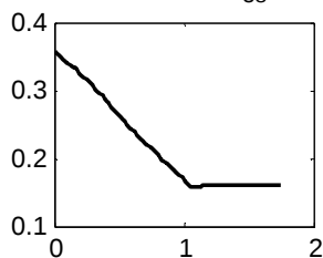
Glucose(N) r_{38}
