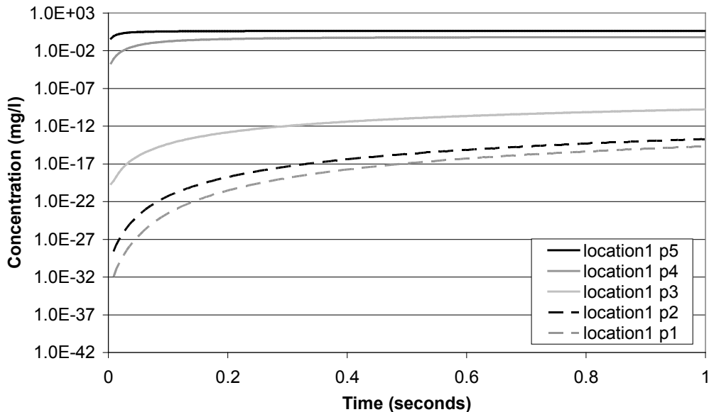
Time evolution of concentration at location #1. Specified Constant Concentration (10 mg/l) Low Outward Pressure Gradient
