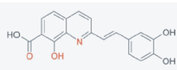
Styrylquinoline
