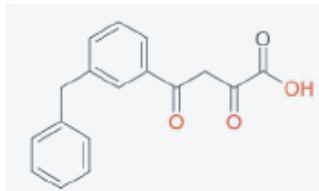
Beta-dicetonic acid
