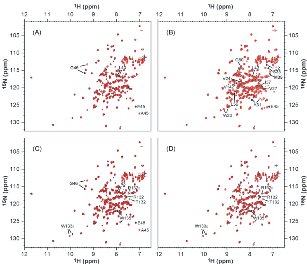
Information for Additional File 1: Figure showing monitoring of structural perturbations of CA-NTD caused by mutations with ^1\text{H} - ^{15}\text{N} HSQC NMR. Superimposed ^1\text{H} - ^{15}\text{N} HSQC spectra of ^{15}\text{N} -labeled wild-type (black) and mutants (red), E45A (A), P38A (B), E45A/R132T (C) and R132T (D). The peaks showing substantial perturbation due to the mutation are labeled with assignments.
