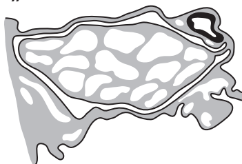
Schizaster canaliferus (from Kaburek & Hilgers 1999)
