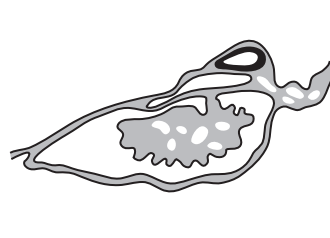
Spatangus purpureus (from Hamann 1887)
