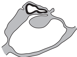
Cidaris cidaris (from Prouho 1887)
