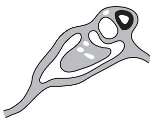
Heterobrissus niasicus (from Wagner 1903)
