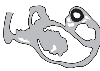
Echinocyamus pusillus (this study)
