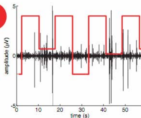
Recording of motor LIFE signals and wavelet denoising
