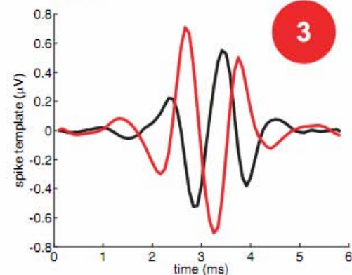
Spike detection and sorting
