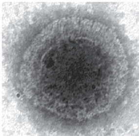
C Virion viral nucleocapsids
