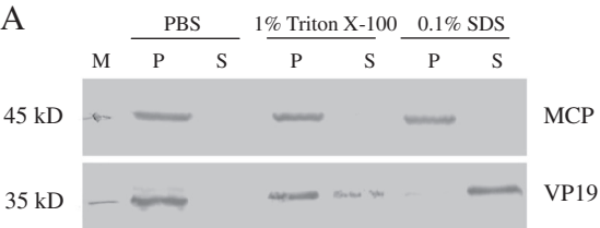
B Virion viral nucleocapsids
