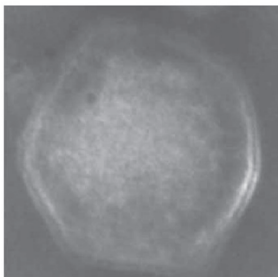
C Virion viral nucleocapsids
