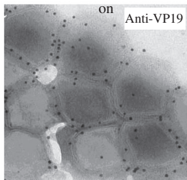
C Virion viral nucleocapsids
