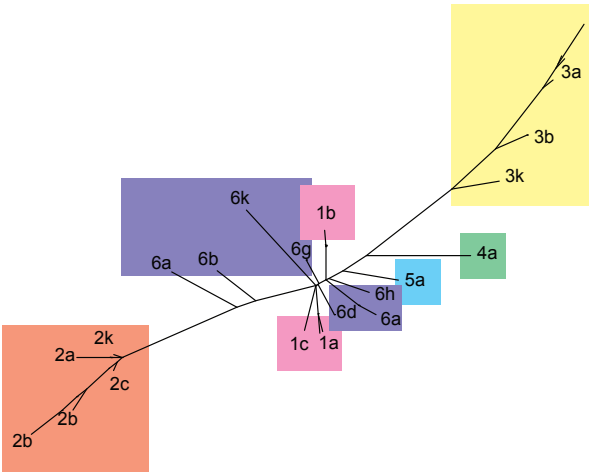
(c) 5' UTR
