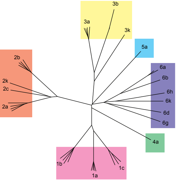
(b) Polyprotein
