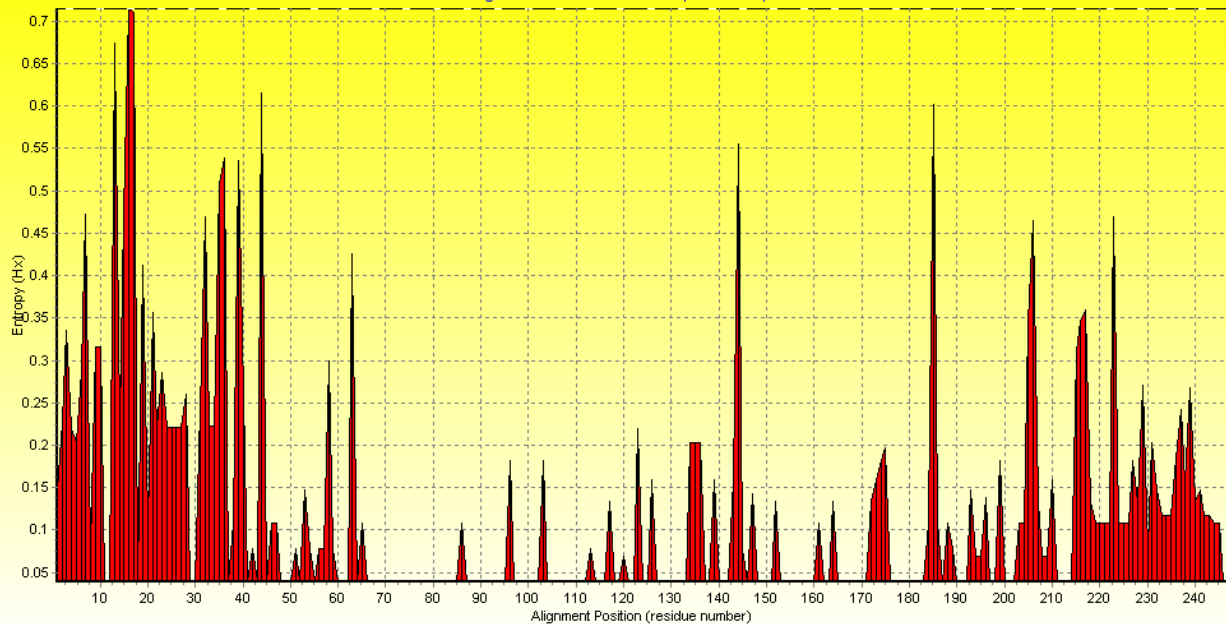
Entropy (Hx) Plot Alignment: C:\BioEdit\Temp\~out.tmp
