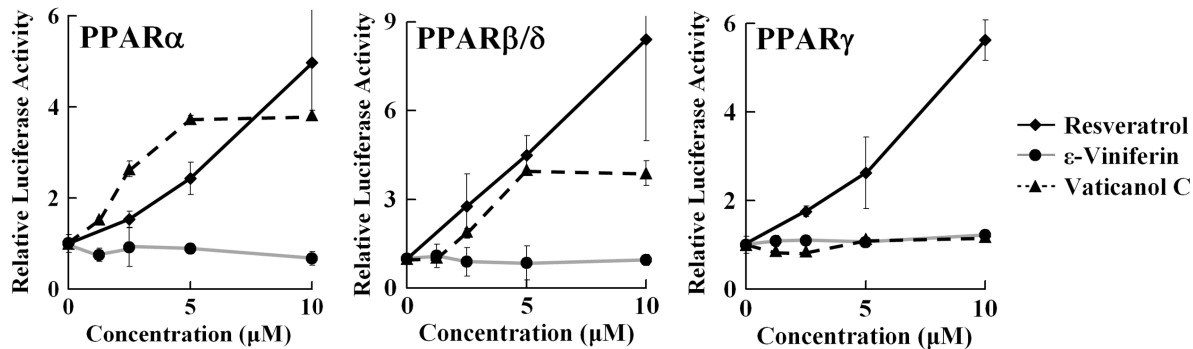
Vaticanol C
