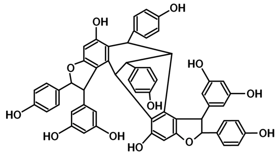
Vaticanol C
