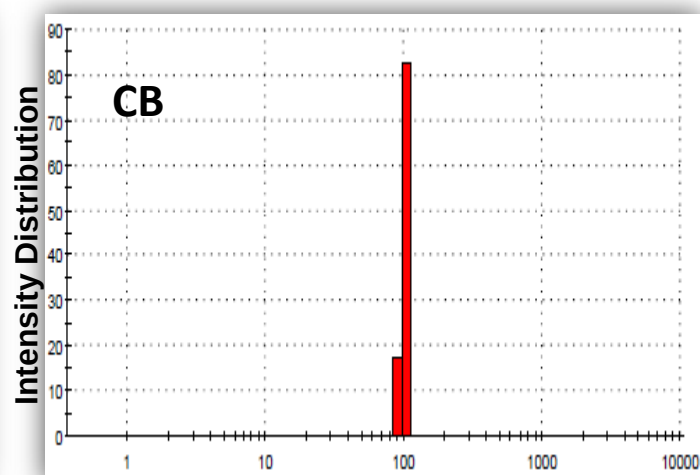
Hydrodynamic Diameter
