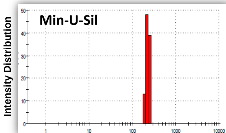
Hydrodynamic Diameter
