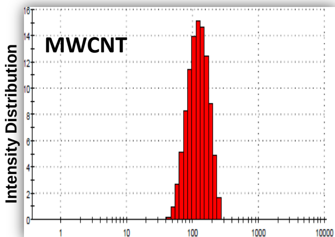
Hydrodynamic Diameter
