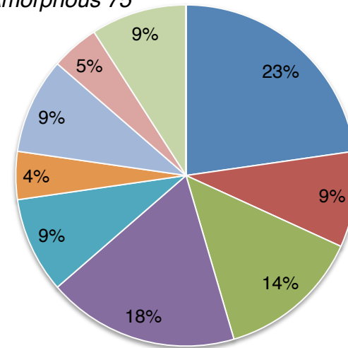
F Amorphous 75
