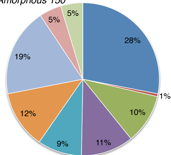
C Amorphous 150
