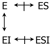
Noncompetitive inhibition ( K_{E_S} = K_{EI_S} )
