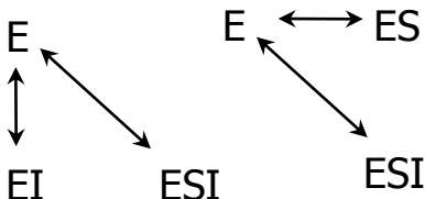
Uncompetitive inhibition
