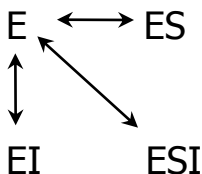
Full spur graph model
