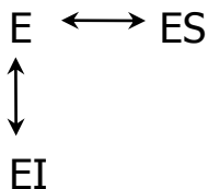
Competitive inhibition
