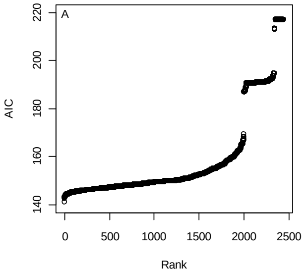
Non-Singular Hessians
