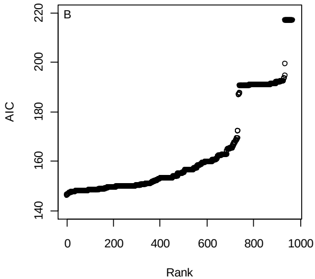
Singular Hessians
