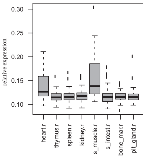
rat: profiles of genes selected based on correlation distance
