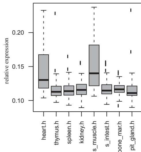
human: profiles of genes selected based on correlation distance
