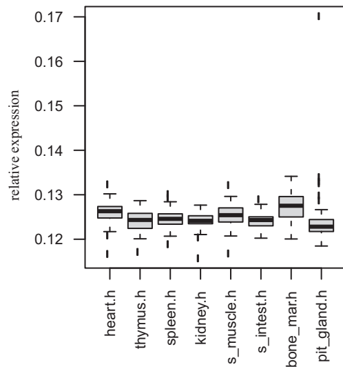
human: profiles of genes selected based on Euclidean distance
