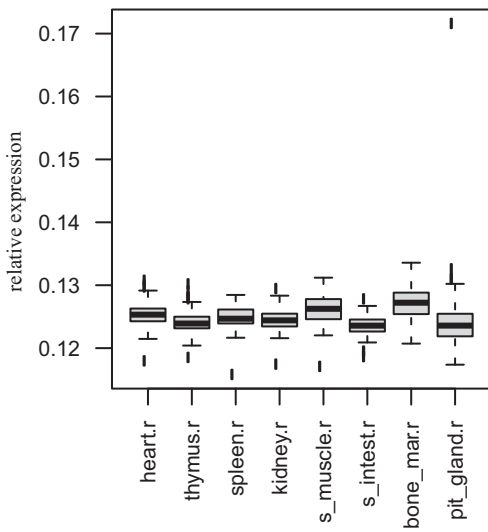
rat: profiles of genes selected based on Euclidean distance
