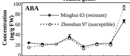
ABA and its biosynthesis-related genes
