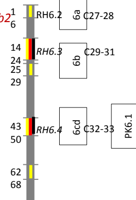
Chromosome 6
