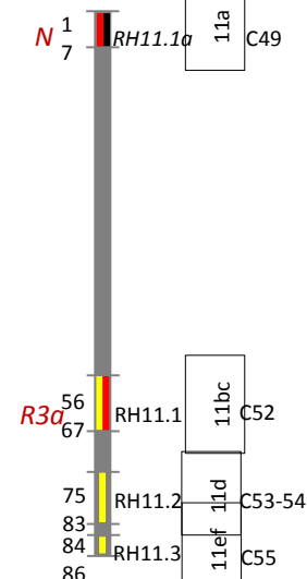
Chromosome 11
