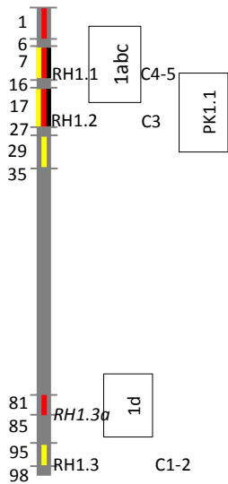
Chromosome 1
