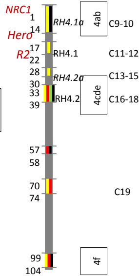
Chromosome 4
