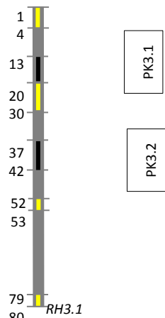
Chromosome 3
