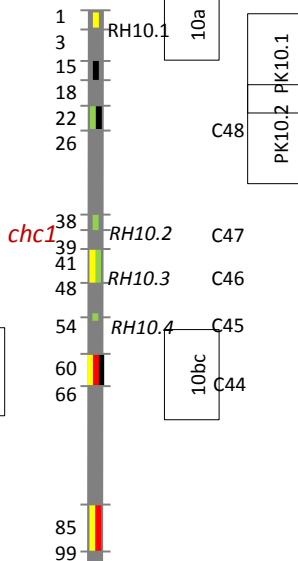
Chromosome 10
