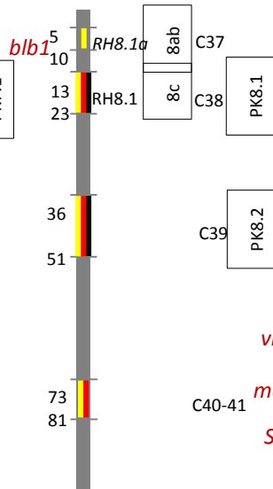
Chromosome 8
