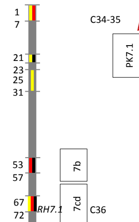
Chromosome 7
