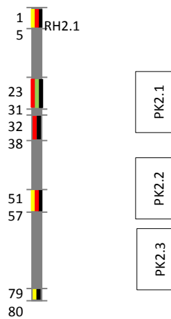
Chromosome 2
