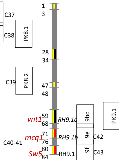
Chromosome 9
