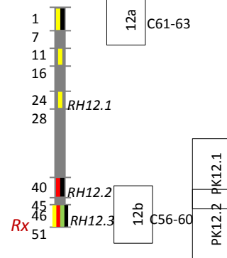
Chromosome 12
