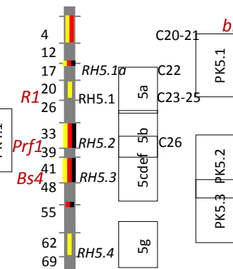
Chromosome 5
