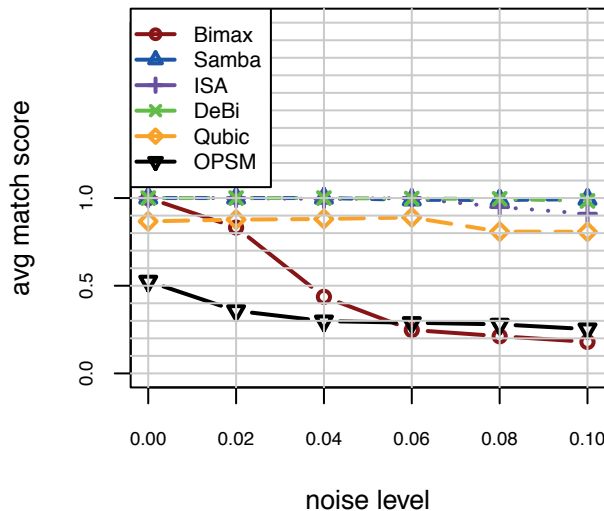
Effect of Noise: Relevance of BC's (Additive)
