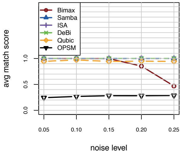
Effect of Noise: Relevance of BC's (Constant)
