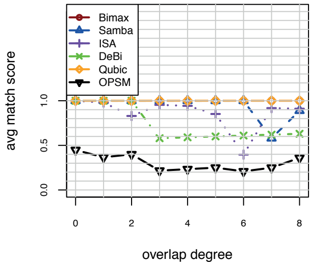
Regulatory Complexity: Relevance of BC's (Constant)
