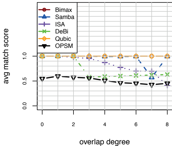
Regulatory Complexity: Relevance of BC's (Additive)
