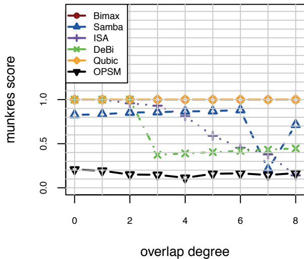
Regulatory Complexity: (Additive)
