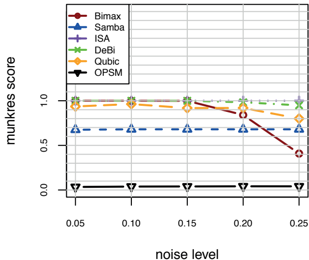
Effect of Noise: (Constant)
