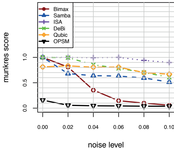
Effect of Noise: (Additive)
