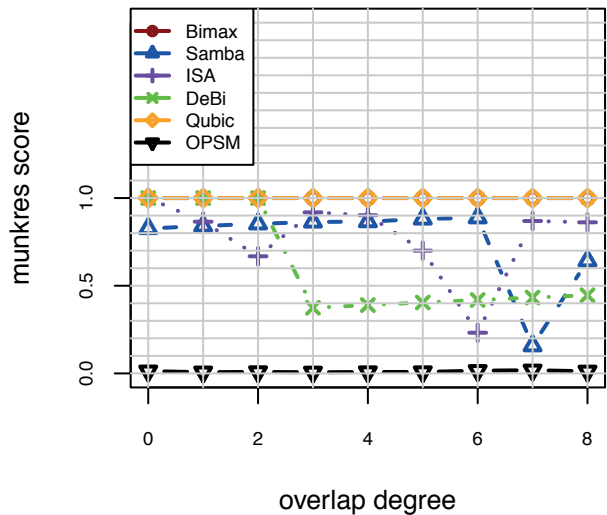
Regulatory Complexity: (Constant)
