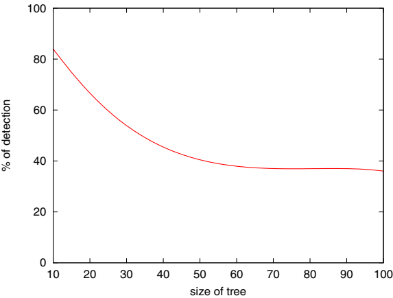
Algorithm performance for 10% misplaced gene insertions
