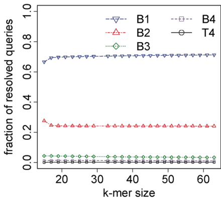
4 Bloom query statistics
