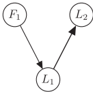
(iv) Reversing an edge (L_2, L_1) to (L_1, L_2) .
