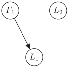
(iii) Deleting an edge (L_2, L_1) .
