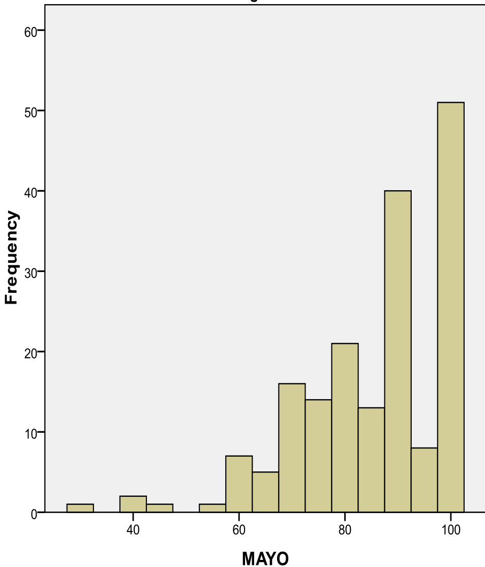
Histogram of the MAYO score
