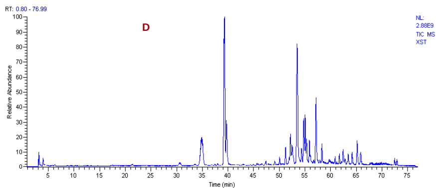
PDA Chromatograms of standard compounds (A) and a XST injection (C), and total ion current chromatograms of standard compounds (B) and a XST injection (D). 1–27 were the characteristic peaks, listed in Table 2 .
