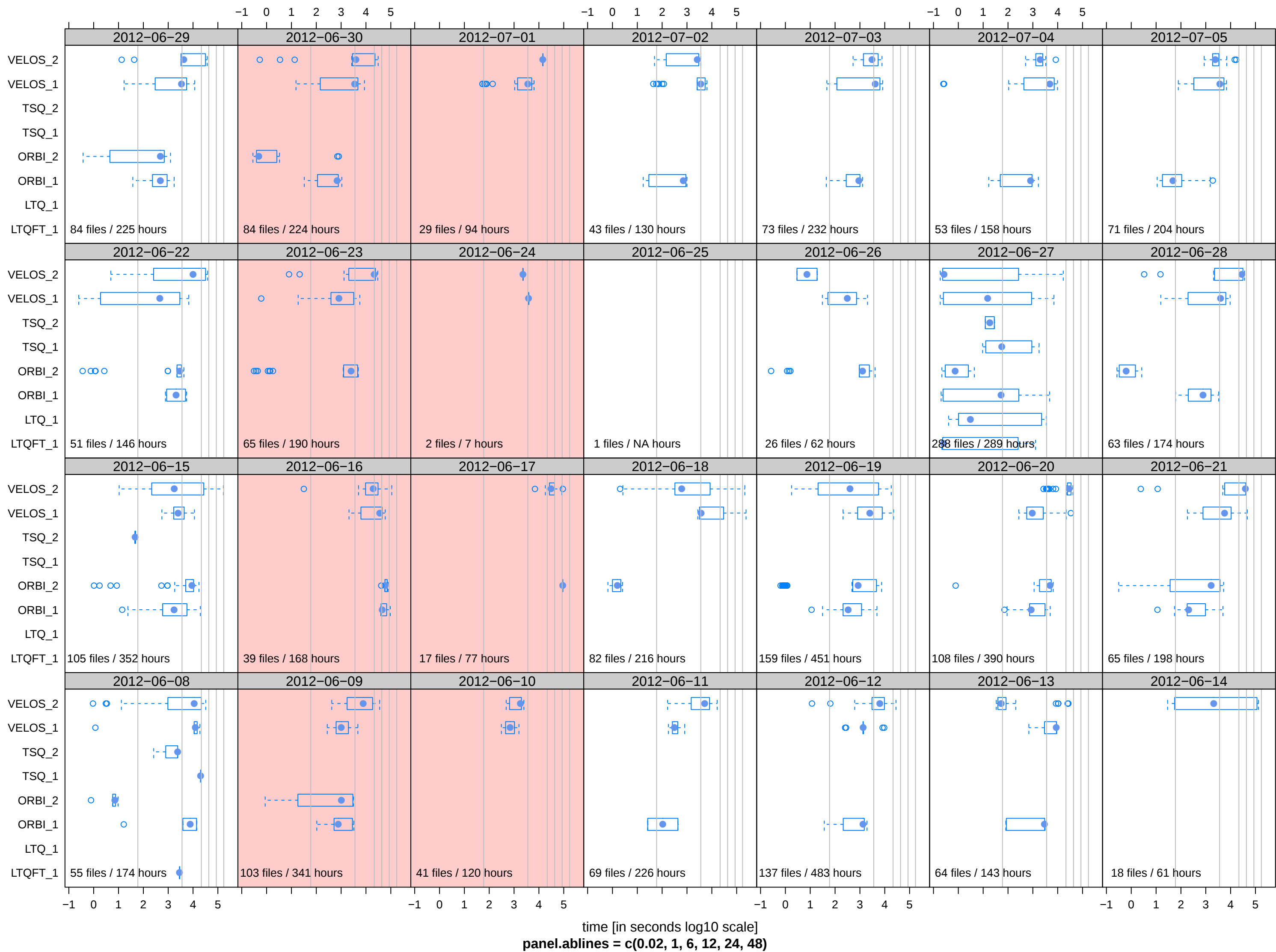
Process time distribution of jobs executed by FCC on daily base.
