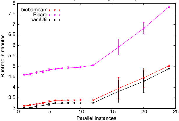
BAM duplicates marking (HG03520)
