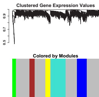
(a) Gene network
