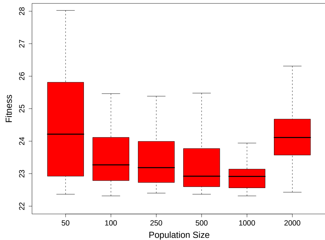
(b) Impact of the population size on the fitness
