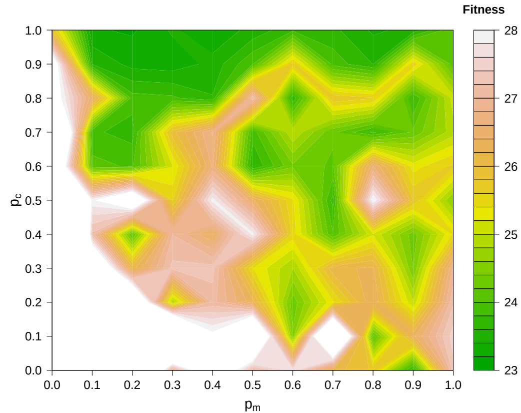
(a) Influence of mutation and crossover probabilities
