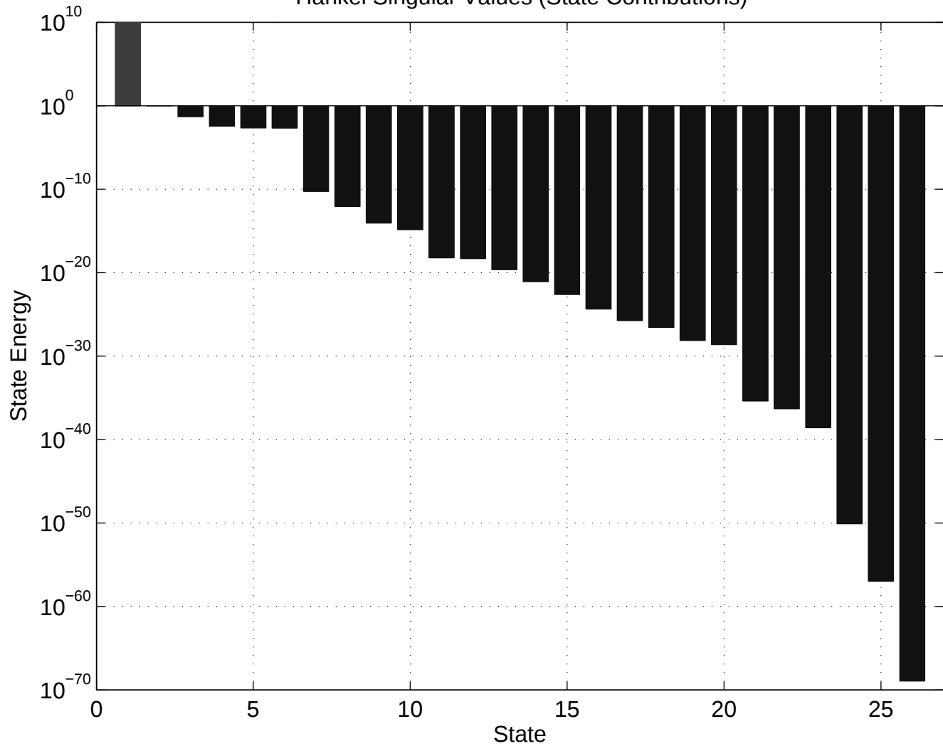
Hankel Singular Values (State Contributions)
