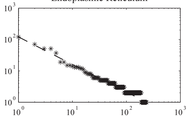
Endoplasmic Reticulum
