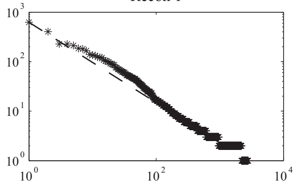
Recon 1
