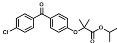
Fenofibrate
