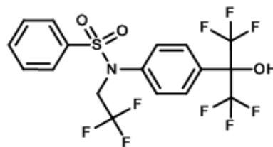
T0901317
