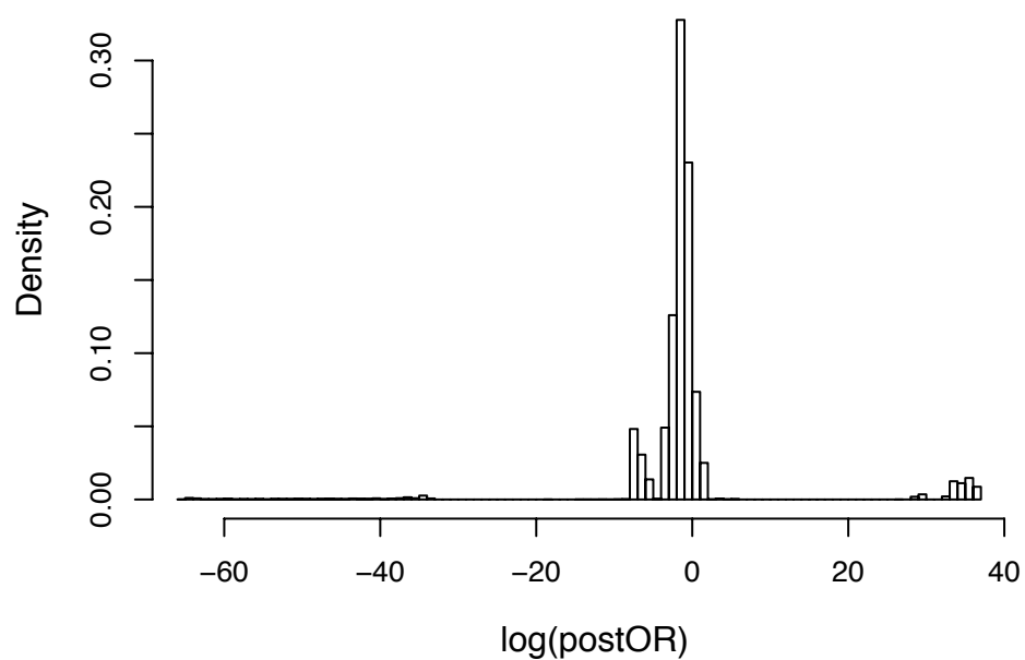
(a) Histogram of log postOR, all edges
