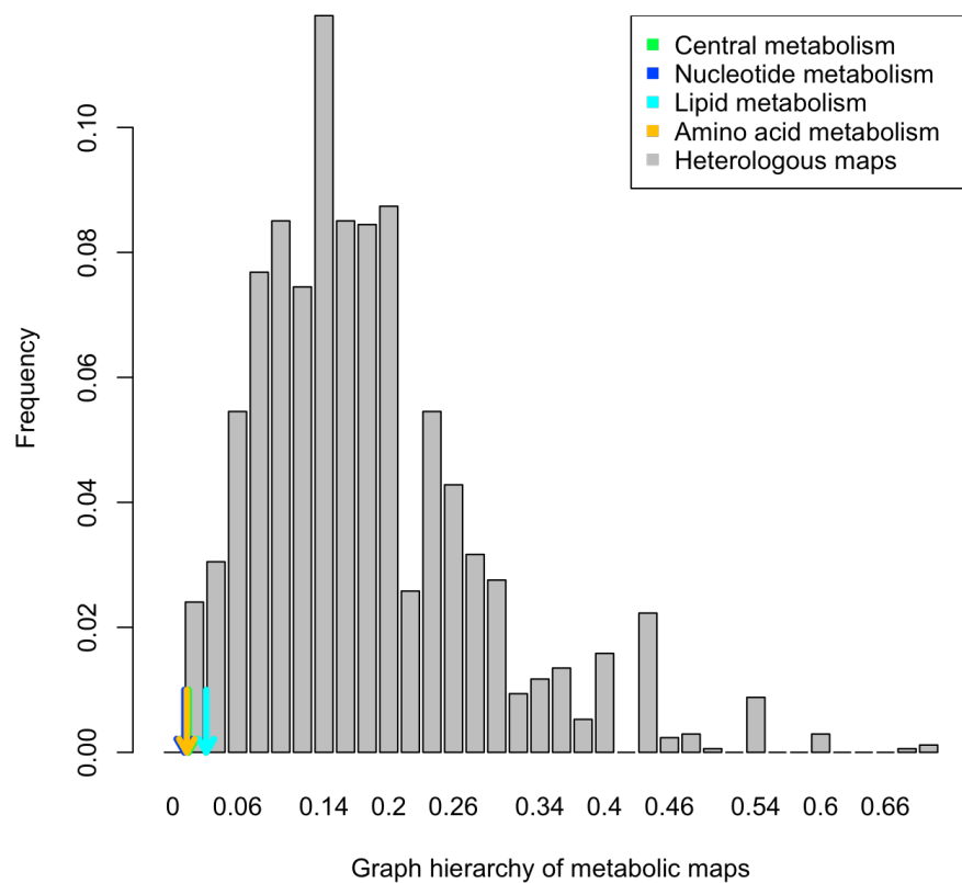
Figure S1: Distribution of graph hierarchies (Butts, C J Stat Soft , 24:1-50, 2008) in heterologous metabolic networks ( 0.169 \pm 0.11 ) in comparison with the graph hierarchy of central (0.032), nucleotide (0.027), lipid (0.051), and amino acid (0.030) metabolic networks in E. coli .
