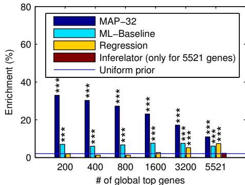
(b) Validating only positive predictions
