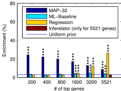
(a) Validating both positive and negative predictions
