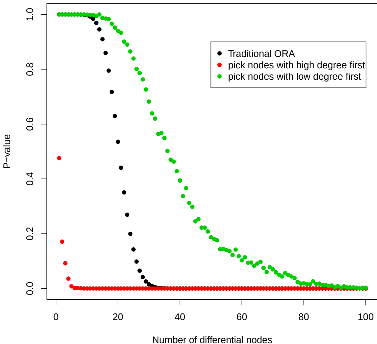
Comparison of p-values influenced by key nodes
