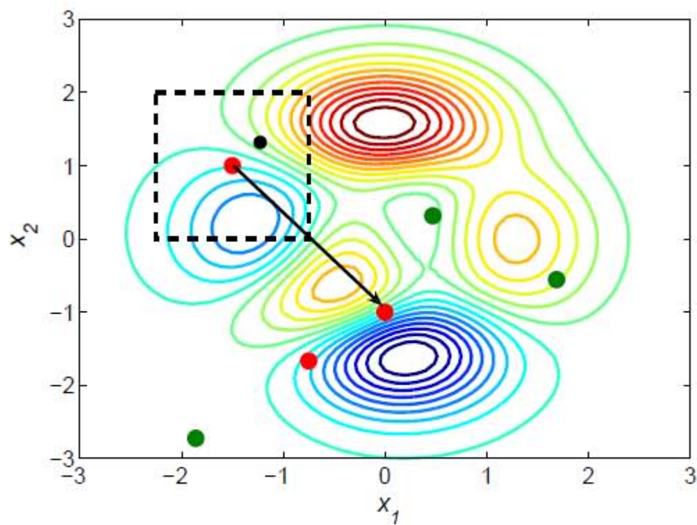
(c) Combination (red solutions) and generation of a new solution (in black)
