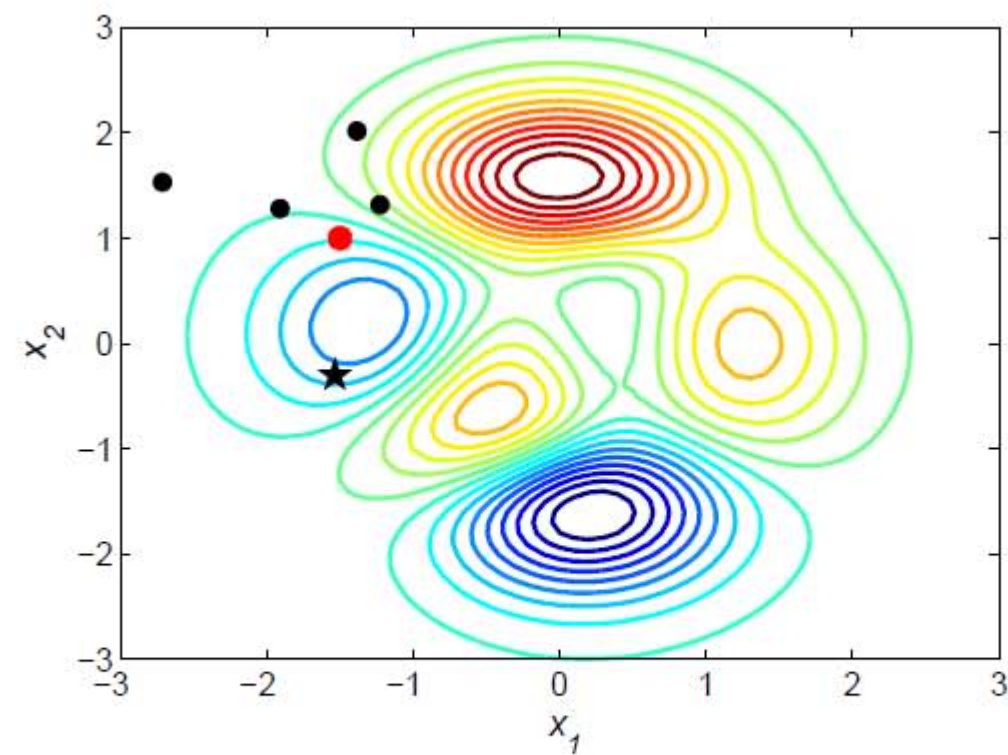
(d) Offspring solutions of a RefSet member
