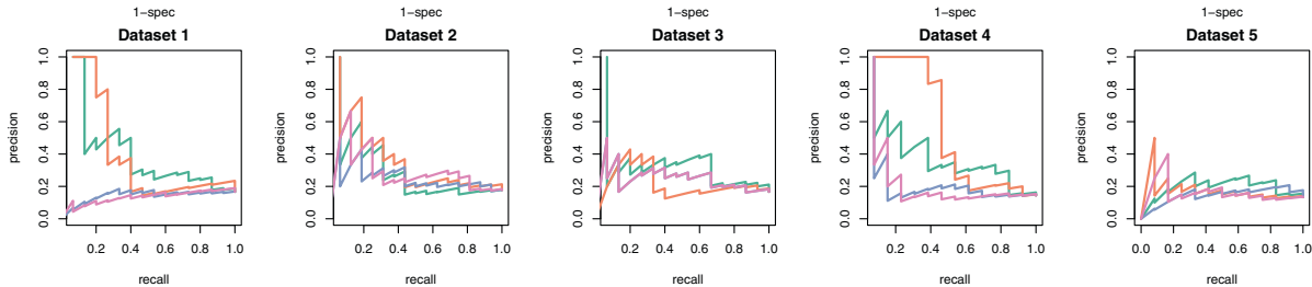
PR curves
