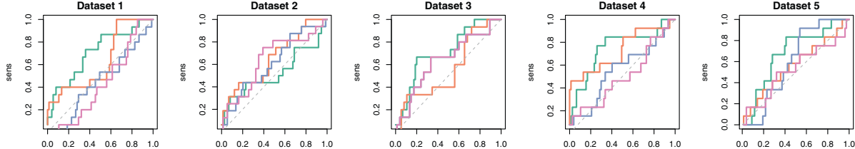
ROC curves
