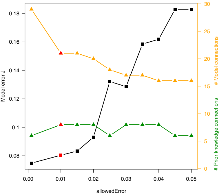
Network model selection
