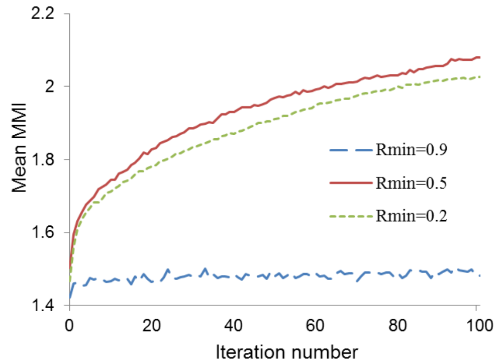
(a) Structure learning
