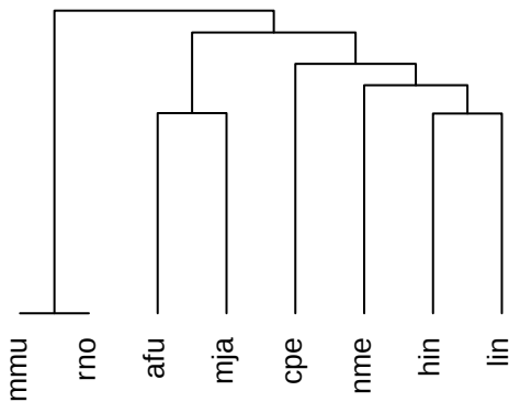
Glycolysis pathway
