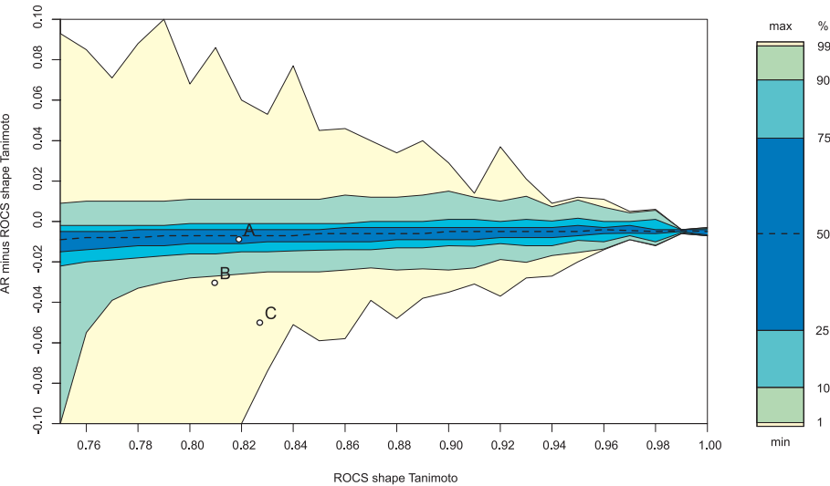
ROCS versus Alignment-Recycling (Transform-Tanimoto=0.73)
